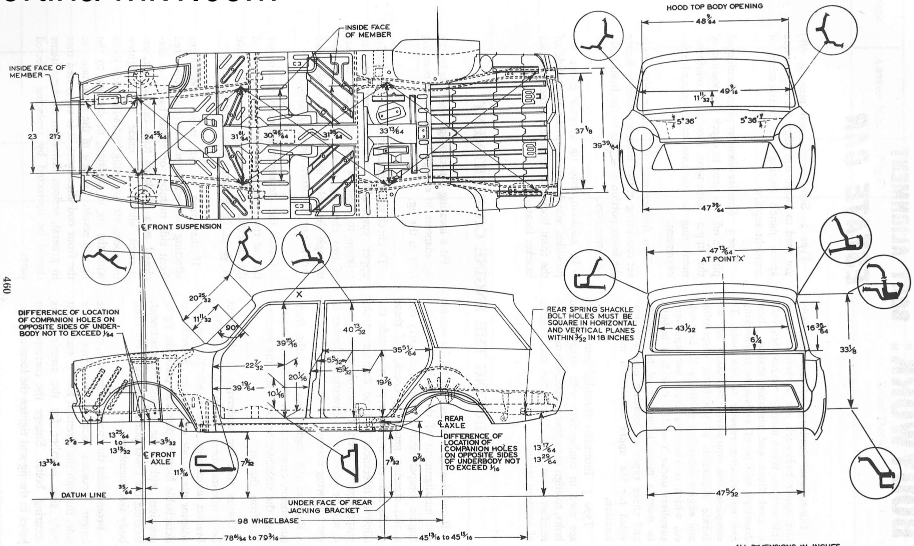
Fig. 1 Consul Cortina Estate Car
